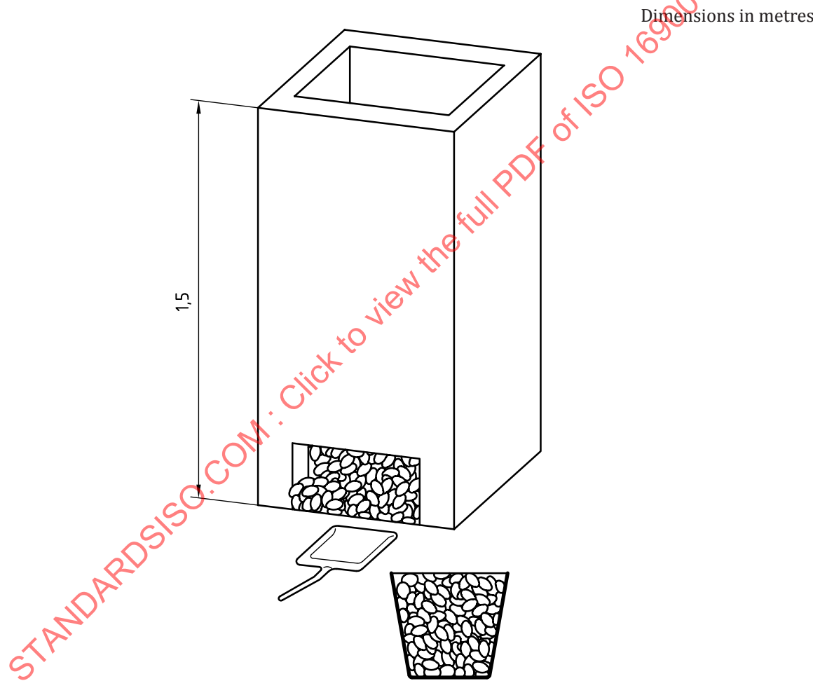
Figure A.1 — Baskets and chippings
