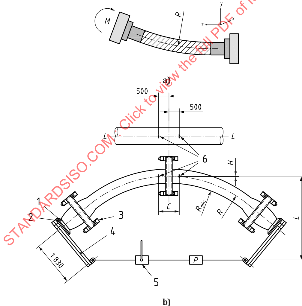
Figure 6 — Principle of the bending stiffness test set up
