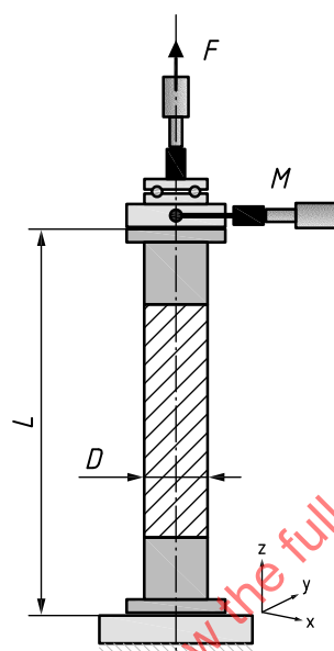
Figure 5 — Principle of the axial tension and torsion test set up
