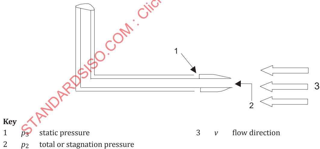
Figure A.2 — Schematic diagram of an L-type Pitot tube
