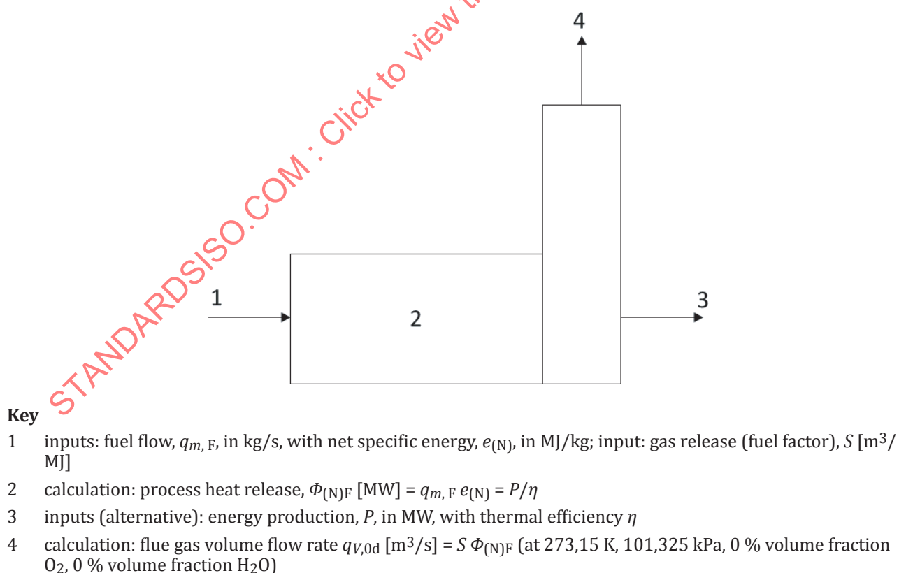
Figure E.1 — Principle of calculation of stack gas flow from energy consumption
