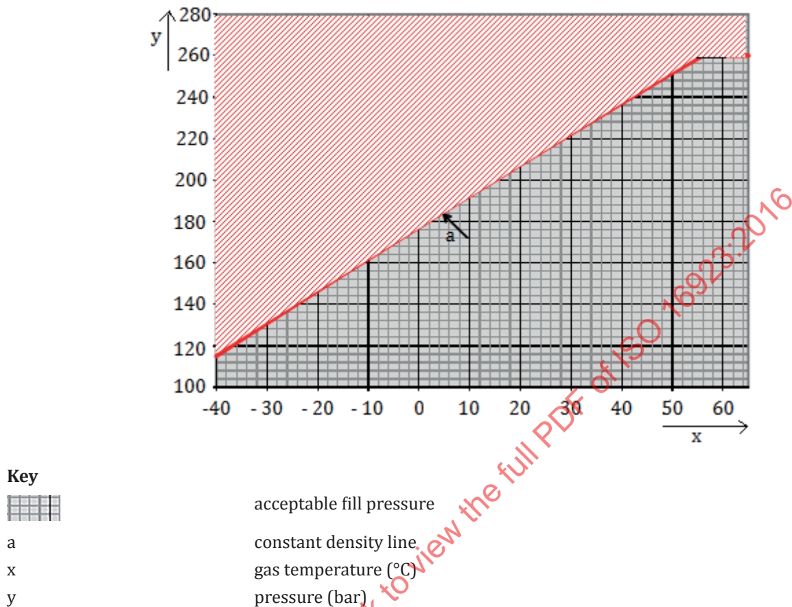
Figure 1 — Temperature compensated fuelling pressure control
