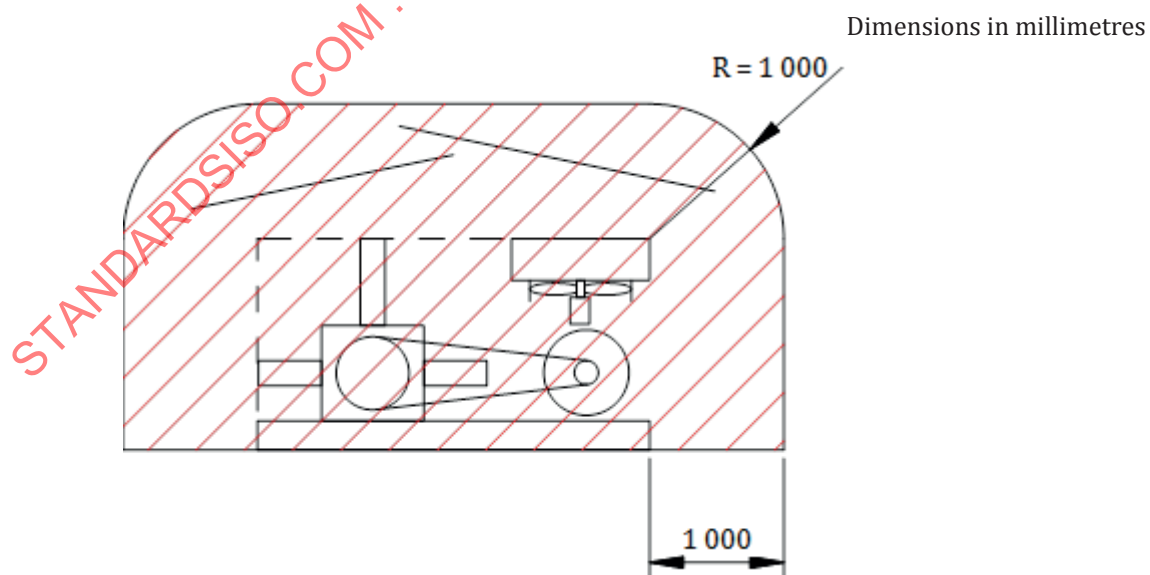
Figure A.2 — Hazardous zones for enclosed and ventilated CNG compressors
