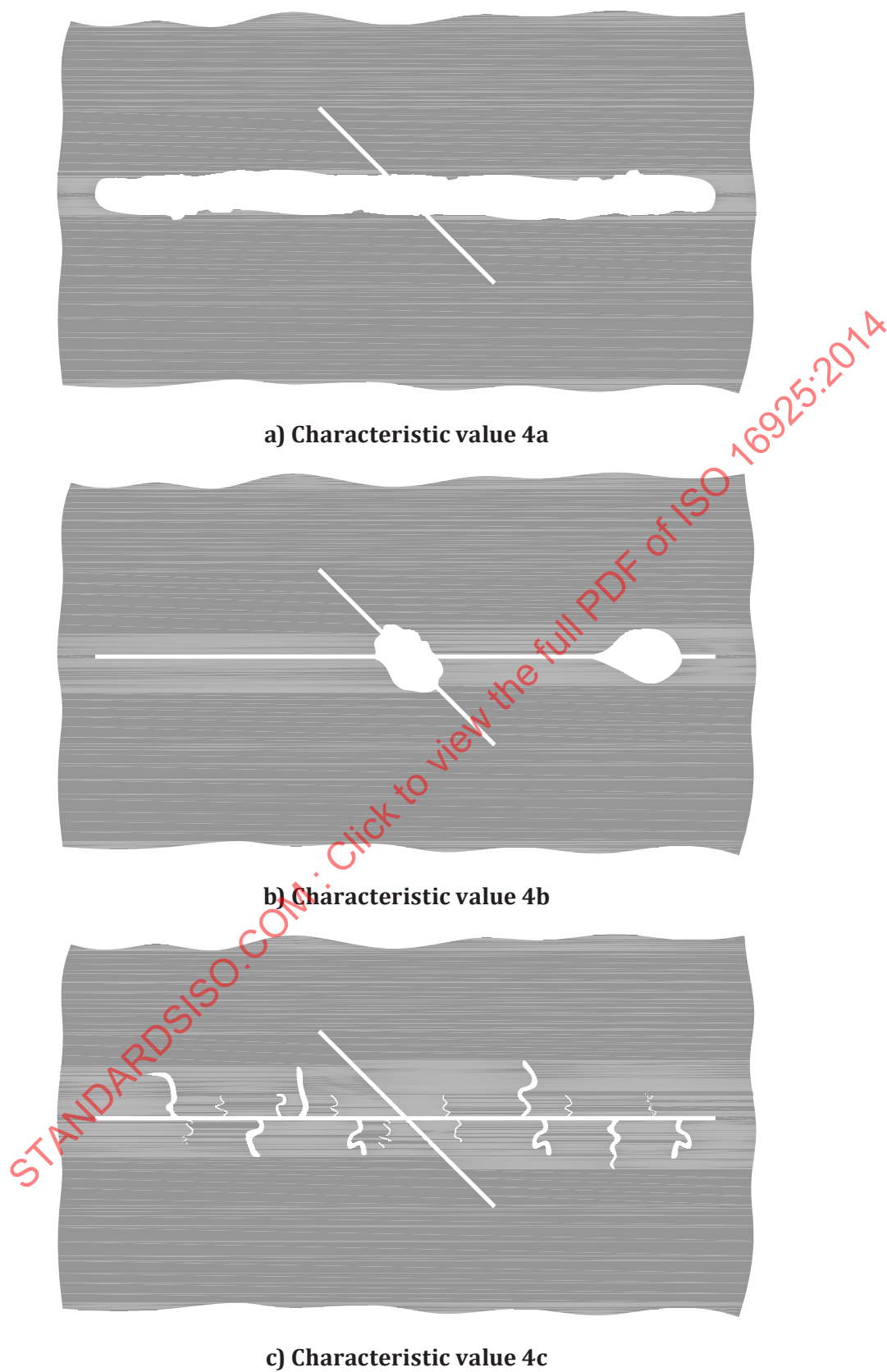
Figure 8 — Characteristic value 4 for pressure water-jet damage
