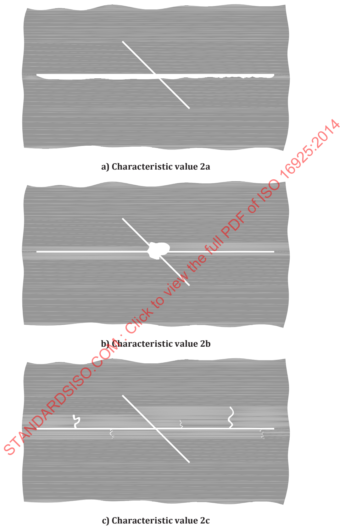
Figure 6 — Characteristic value 2 for pressure water-jet damage
