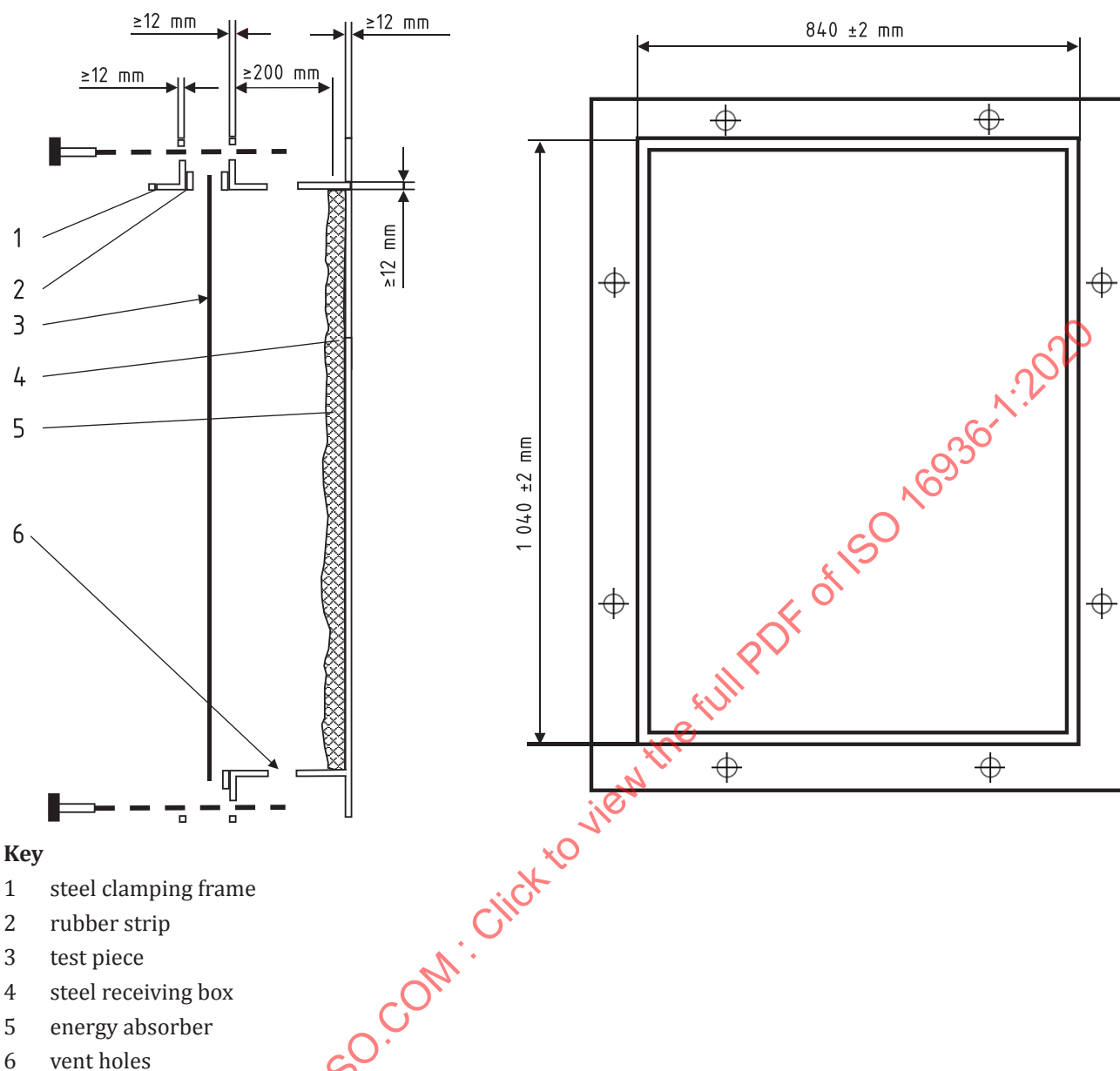
Figure 1 — Example of a test piece support apparatus
