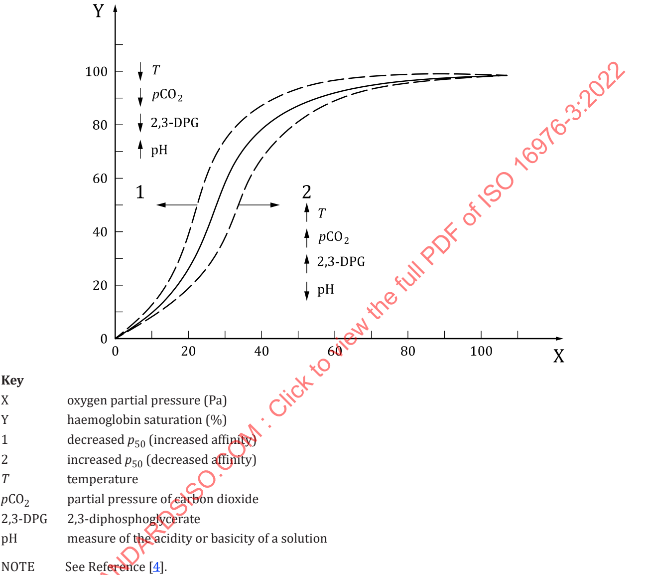
Figure 1 — Shift of the oxyhaemoglobin dissociation curve by pH, carbon dioxide, temperature, and 2,3-diphosphoglycerate (2,3-DPG)
