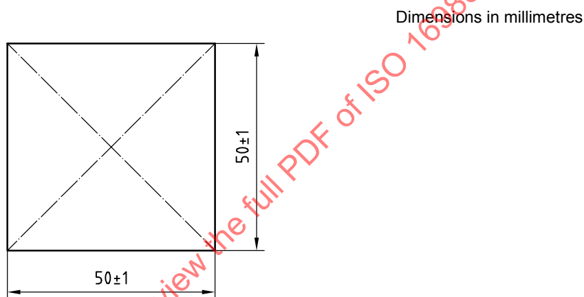
Figure 1 — Test piece for the measurement of swelling in thickness
