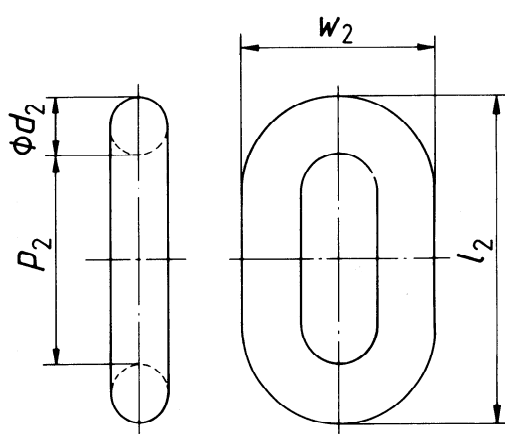
Figure 3 — End link
