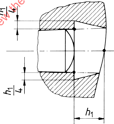
Detail of dovetail chamber for retaining pellet
