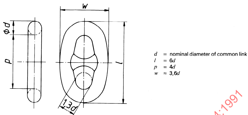
Figure 1 — Common link
