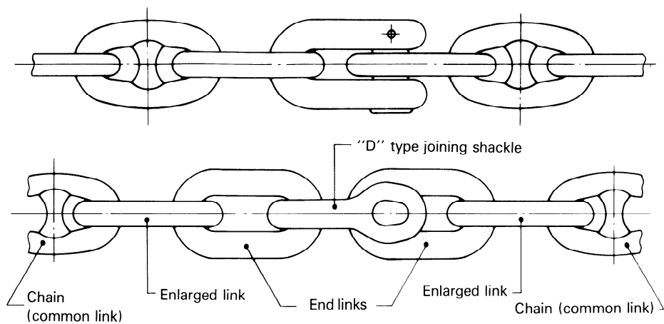
a) Example of joining chain-strands with "D" type joining shackle
