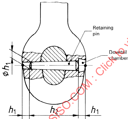
Detail of tapered retaining pin
