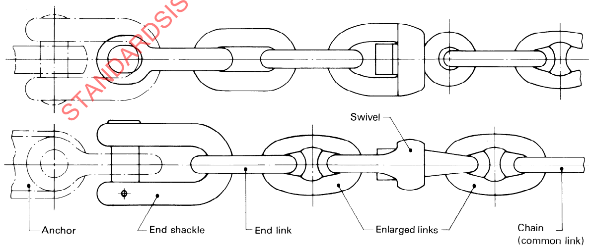
c) Example of connecting chain to anchor
