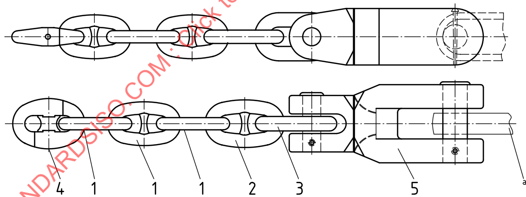
Figure 10 — Examples of connecting chain-shots with a joining shackle
