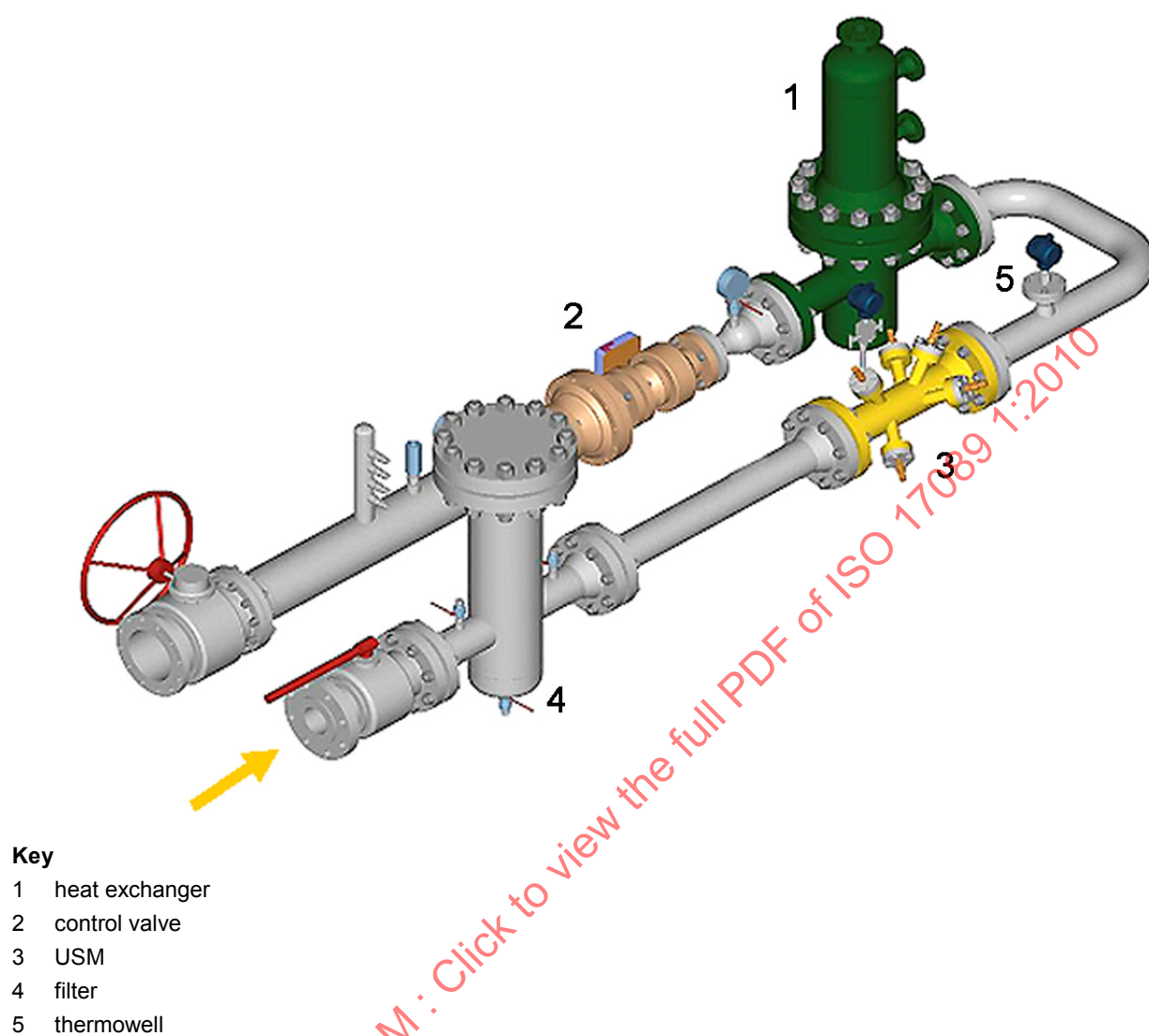
Figure 18 — M&R station optimized for ultrasonic measurement
