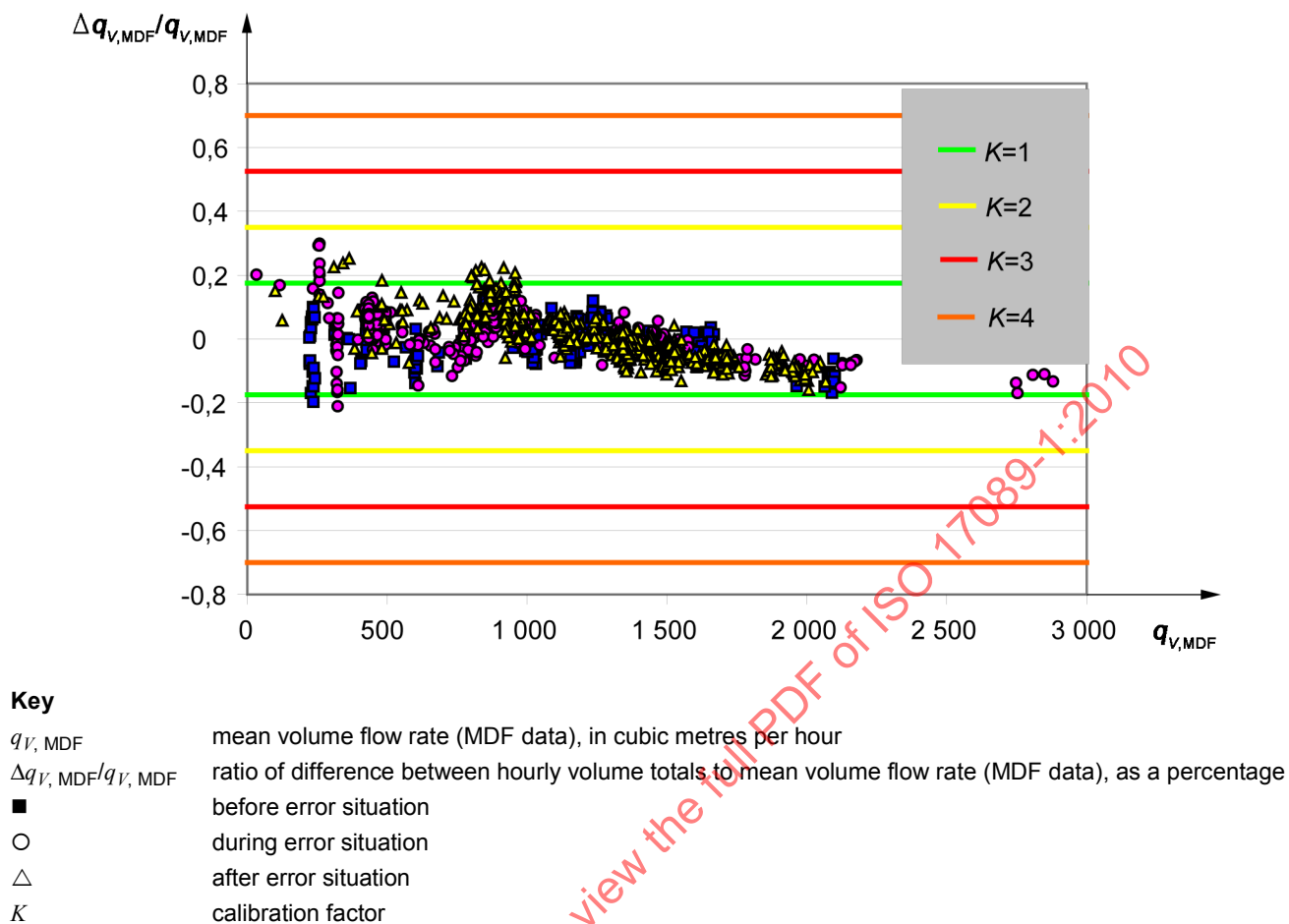
Figure C.5 — Comparing monthly difference footprints (MDF) before, during and after error situation
