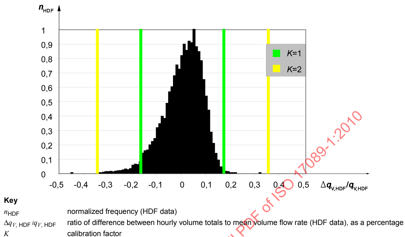
Figure C.3 — Historic difference histogram (HDH)
