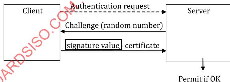
Figure B.1 — Authentication procedure in a simple challenge and response mechanism
