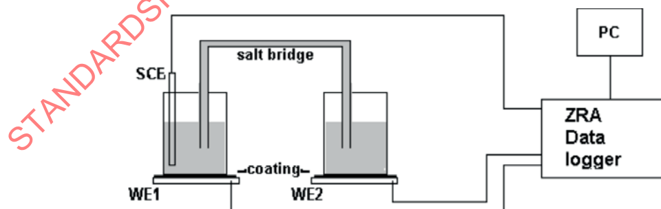
Figure C.1 — EN measurement setup (WE1 and WE2 = working electrode(s), SCE = saturated calomel electrode as the reference electrode)
