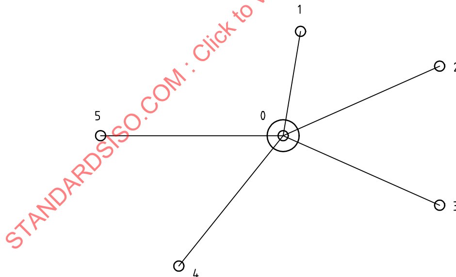
Figure 1 — Test configuration for measurement of horizontal directions
