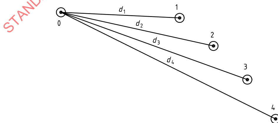
Figure 1 — Configuration of the test field for the simplified test procedure
