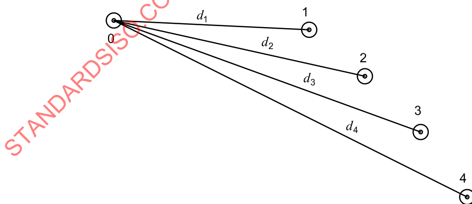
Figure 1 — Configuration of the test field for the simplified test procedure
