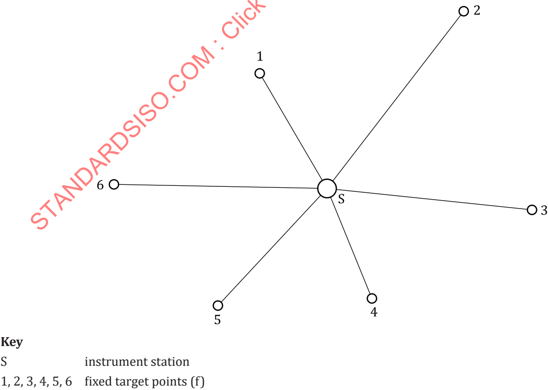
Figure 2 — Configuration of the test field for the simplified test procedure
