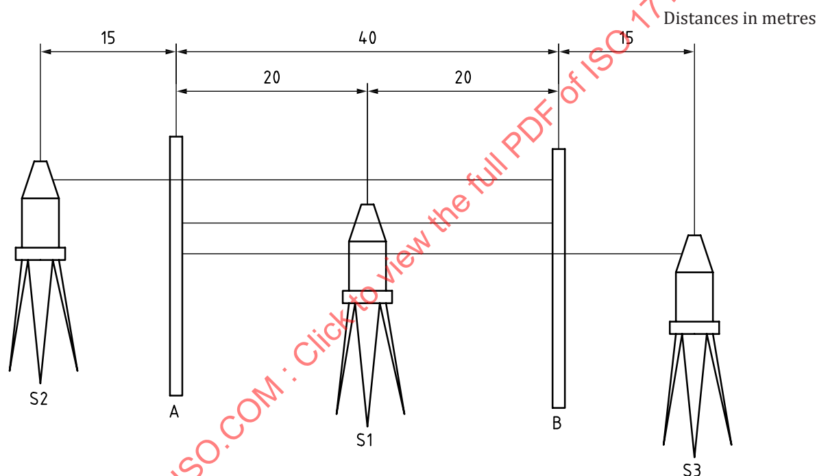
Figure 3 — Example of a configuration of the test line for the full test procedure
