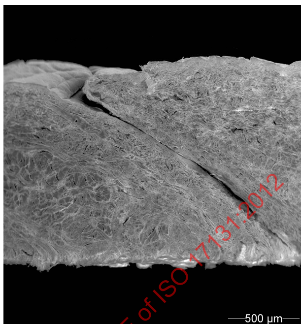
Figure A.4 — Typical section of pig skin leather
