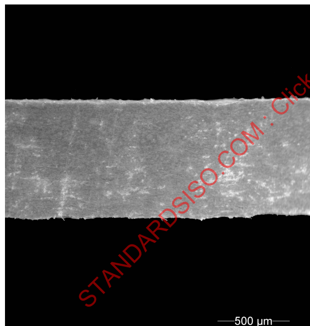
a) Section of a leather fibre board material with moderate magnification
