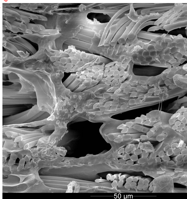
b) Section of a microfibre material with high magnification
