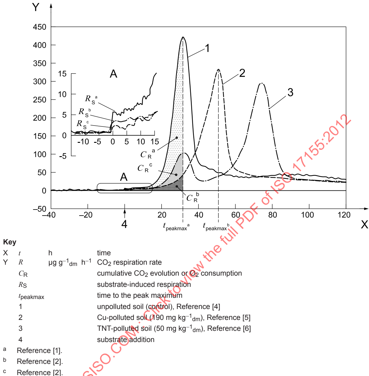
Figure 2 — Soil respiration curves of an unpolluted and two polluted soils
