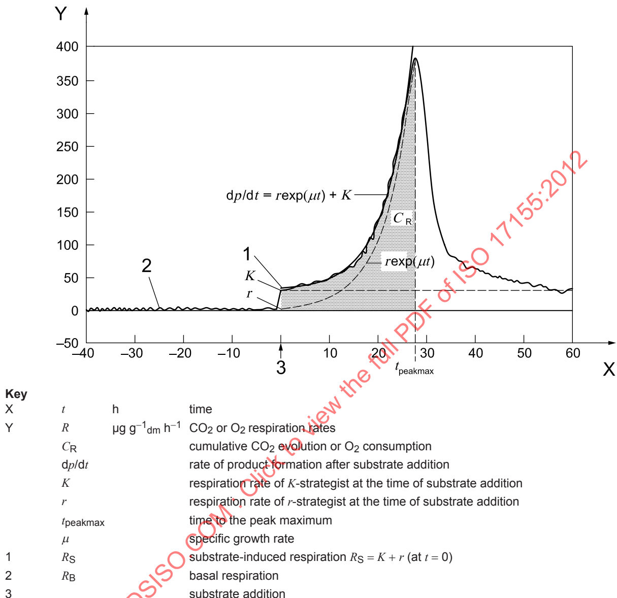
Figure 1 — Soil respiration rate before and after addition of an easily degraded substrate
