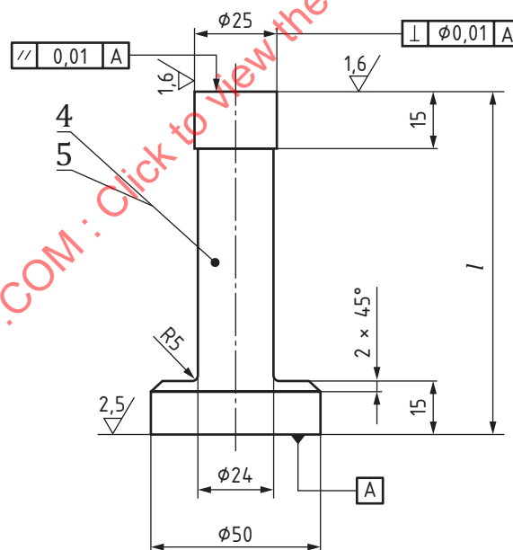
(b) Upper and lower punch
