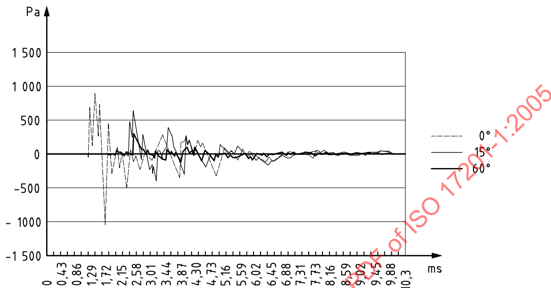
Figure B.1 — Measured sound pressure at 0°, 15° and 60° for 0,67 m chocked barrel, 24 g pellets and muzzle speed 400 m/s
