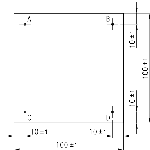
Figure 1 — Location of measurement reference points on a test piece (all dimensions in millimetres \pm 1 mm)
