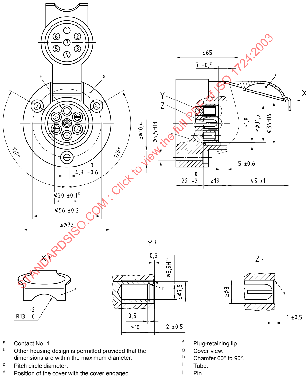
Figure 2 — Socket
