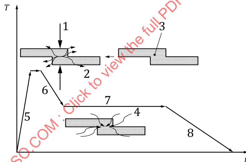
Figure 7 — Cycle of oxygenation-annealing process under pressurized oxygen environment in oxygenation-annealing chamber
