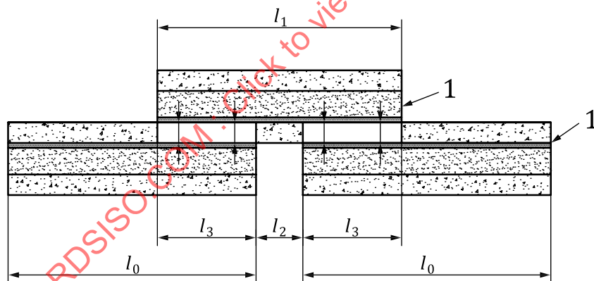
Figure C.1 — Lap joint
