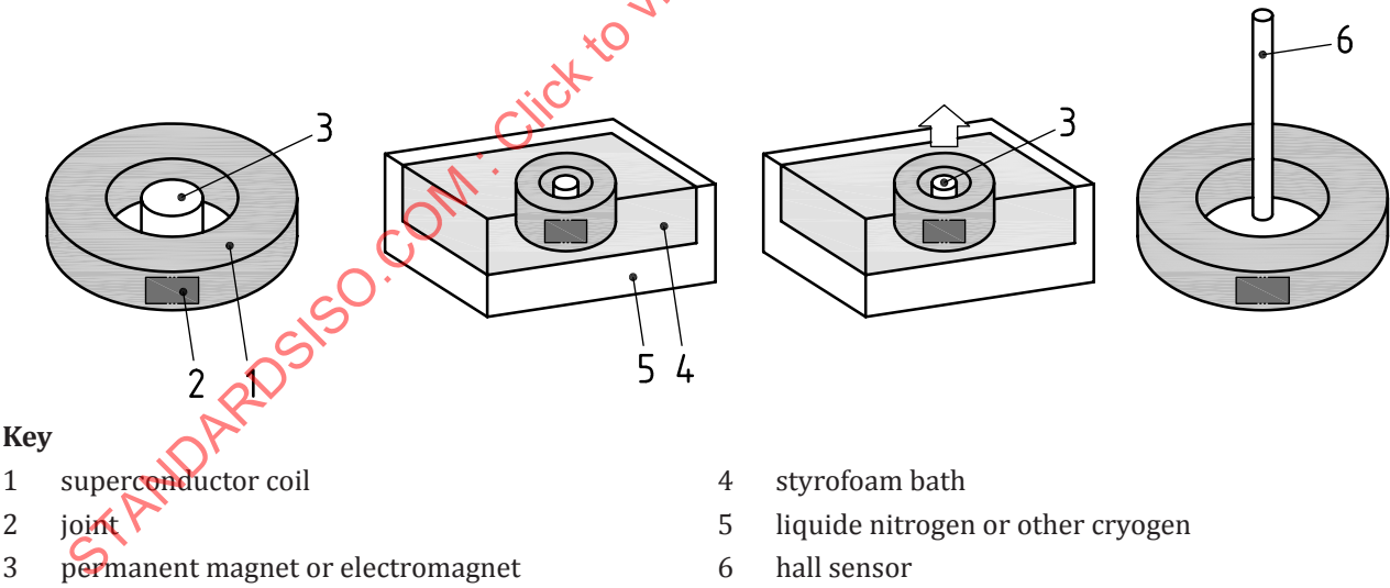
Figure C.2 — Field-decay testing
