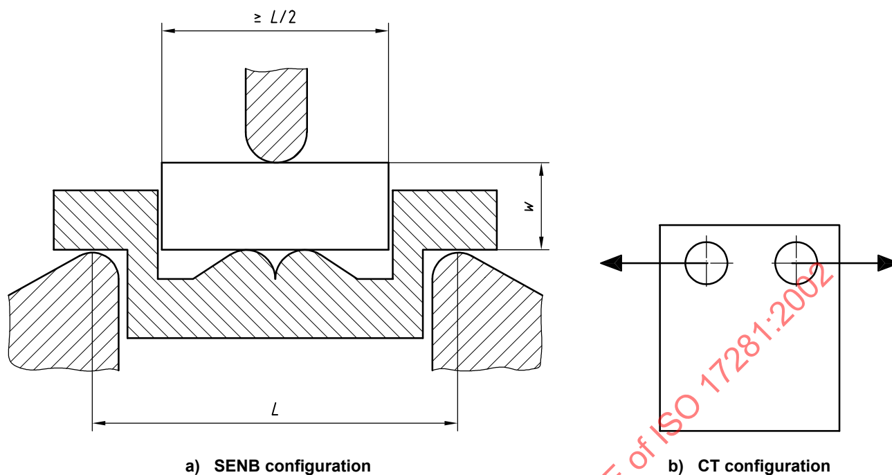
Figure 7 — Arrangements for the energy correction test
