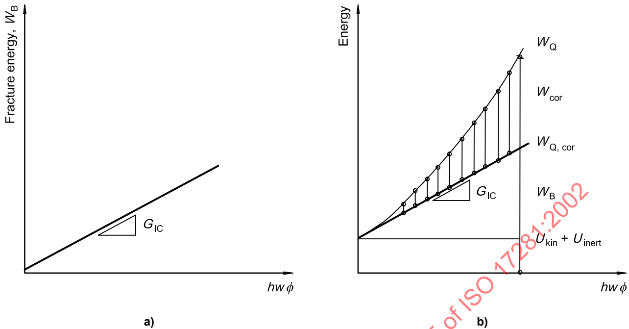
Figure 9 — Determination of G_{IC} from:
