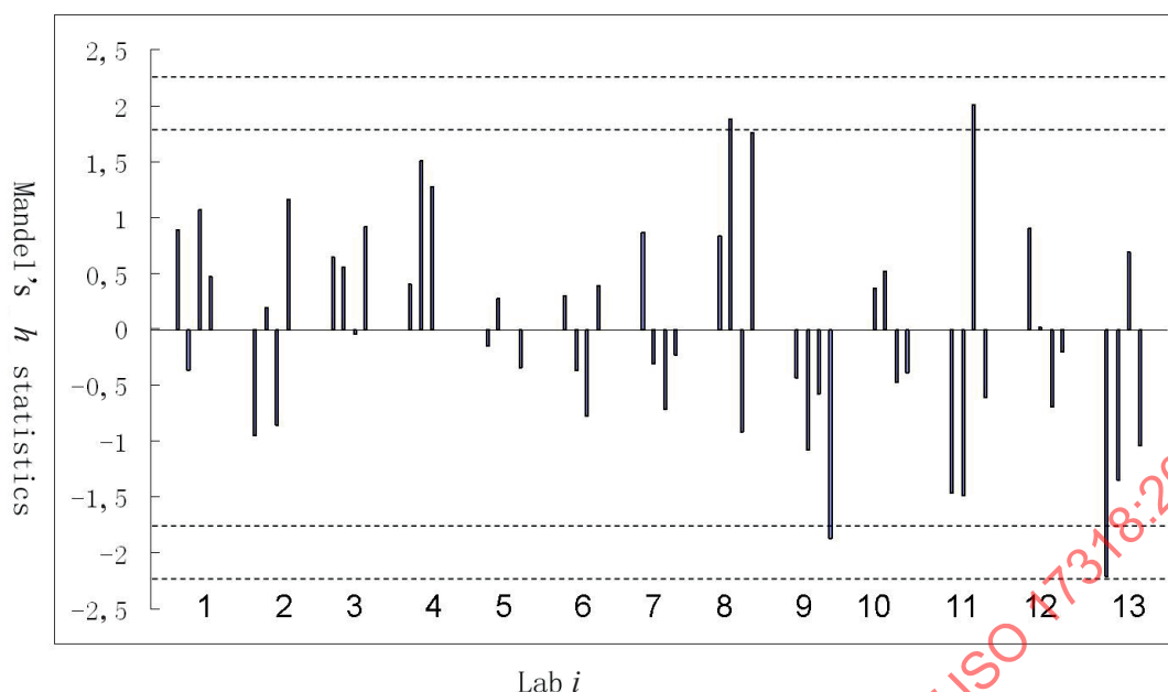
Figure 7 — Mandel's between-laboratory consistency statistic, h , grouped by laboratories
