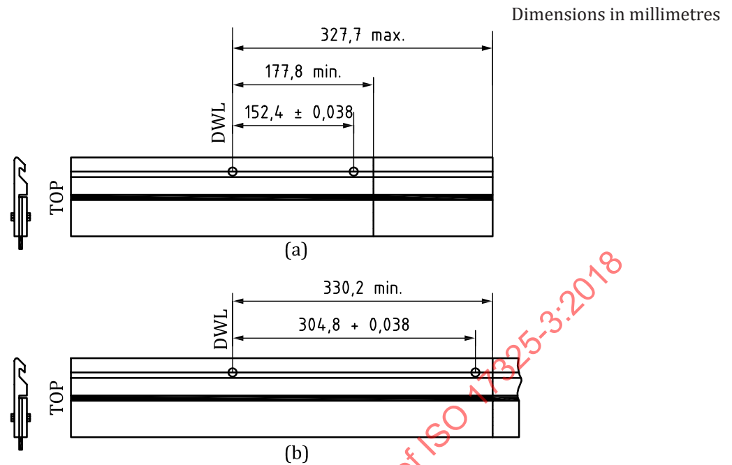
Figure 7 — Connector hole location including self-locking pin
