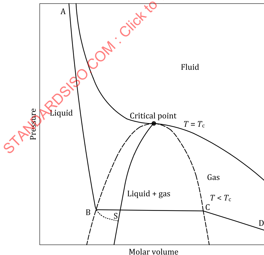
Figure F.1 — Variation of pressure with volume occupied at constant temperature and equilibrium
