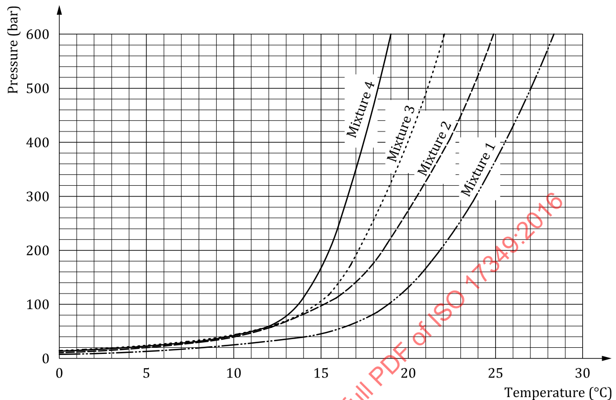
Figure B.2 — Hydrate stability zones for CO 2 /HC mixtures
