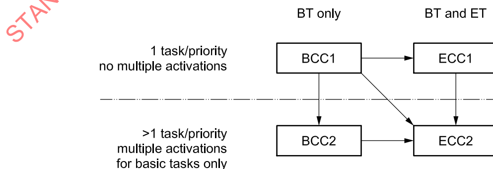
Figure 3 — Restricted upward compatibility for conformance classes
