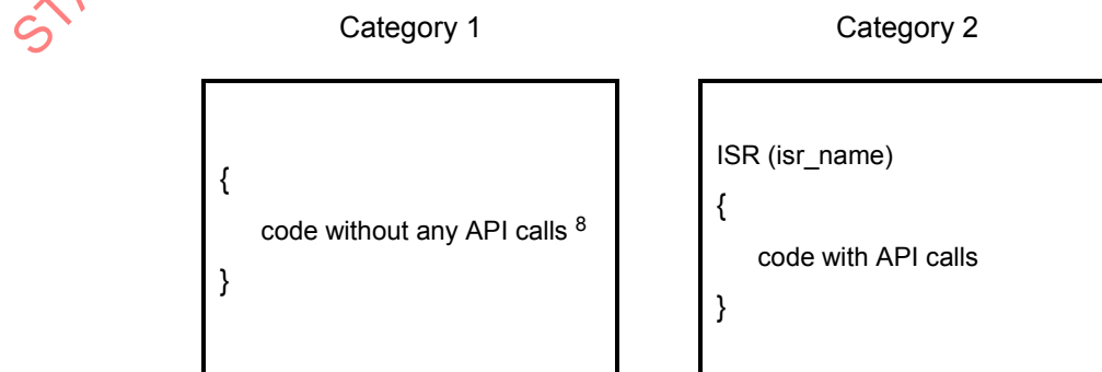
Figure 9 — ISR categories of the operating system
