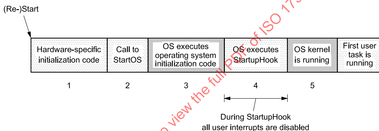
Figure 19 — System start-up
