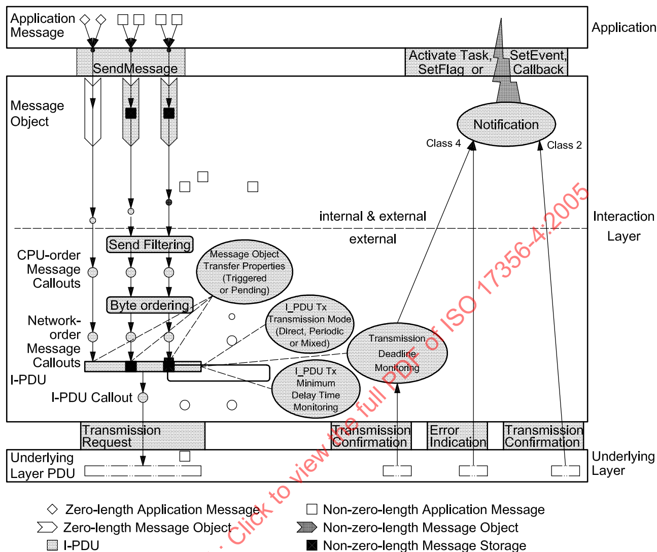
Figure 20 — IL model for external transmission
