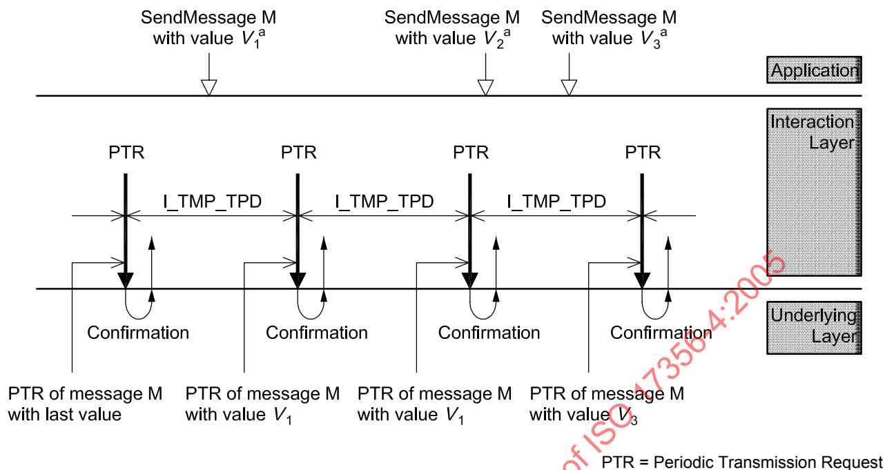
Figure 6 — Periodic Transmission Mode
