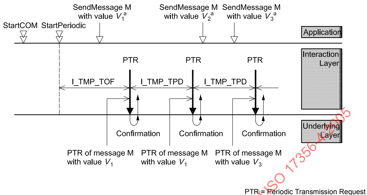
Figure 9 — Activation of the periodic transmission mechanism (example for an I-PDU with Periodic Transmission Mode)
