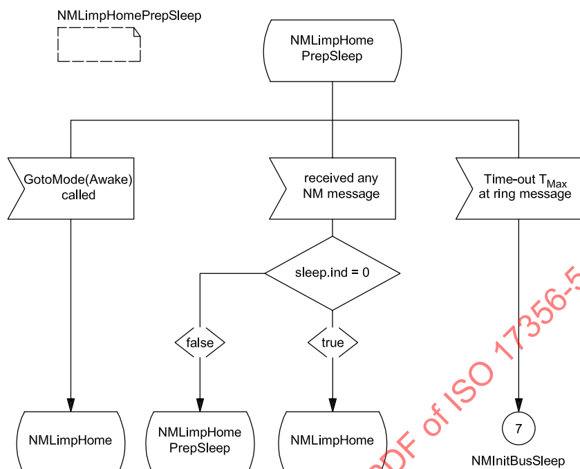
Figure 36 — NMLimpHomePrepSleep
