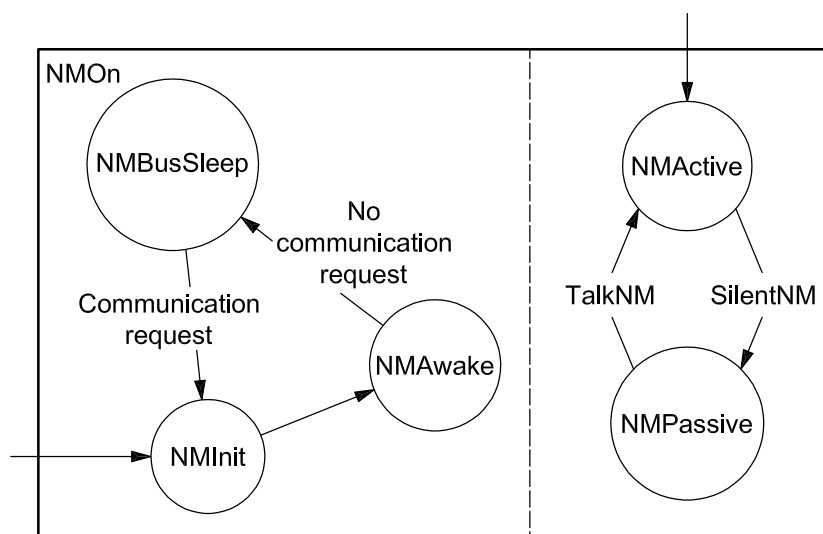
Figure 20 — Toggling between NMAwake and NMPassive
