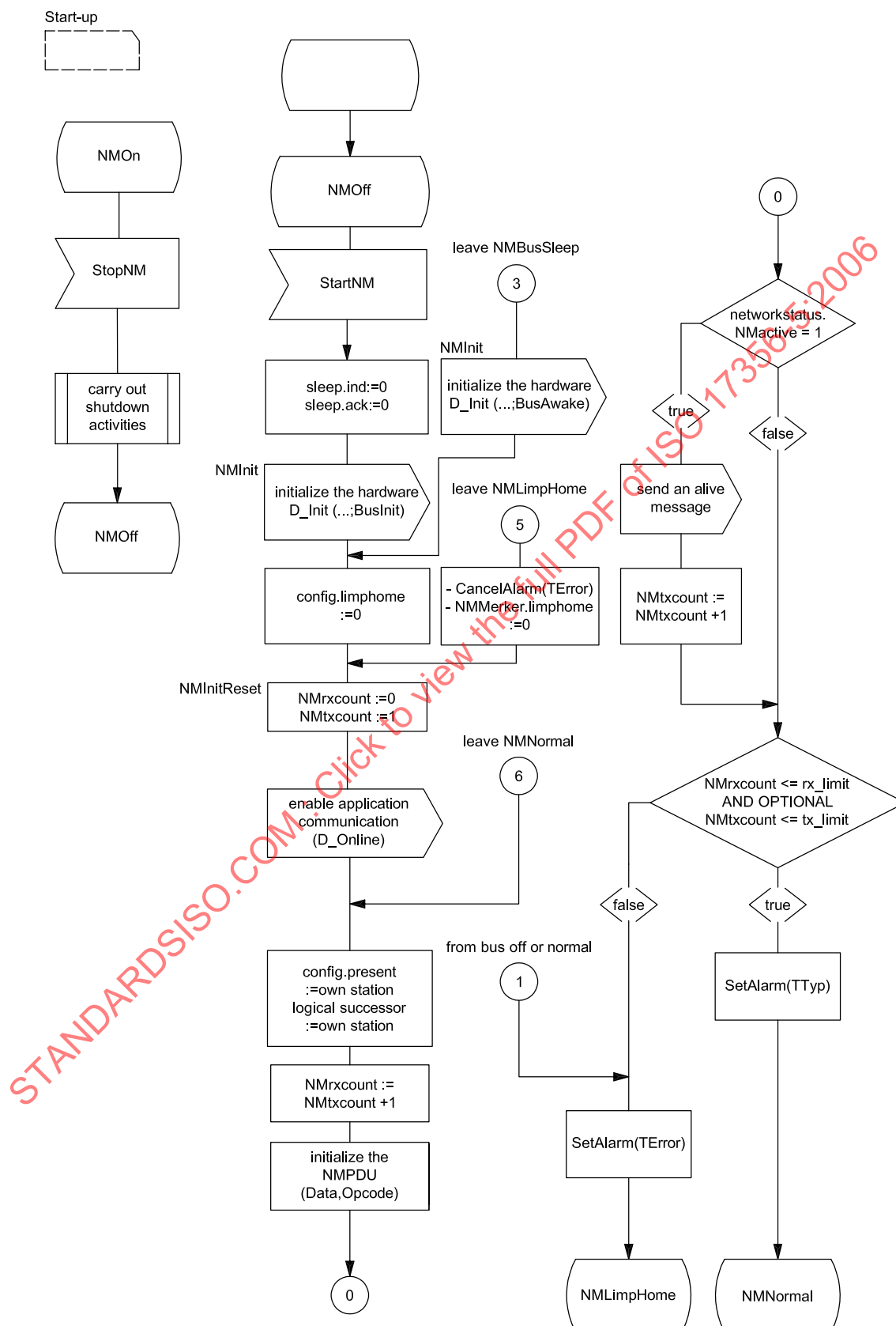
Figure 30 — Start-up of the network
