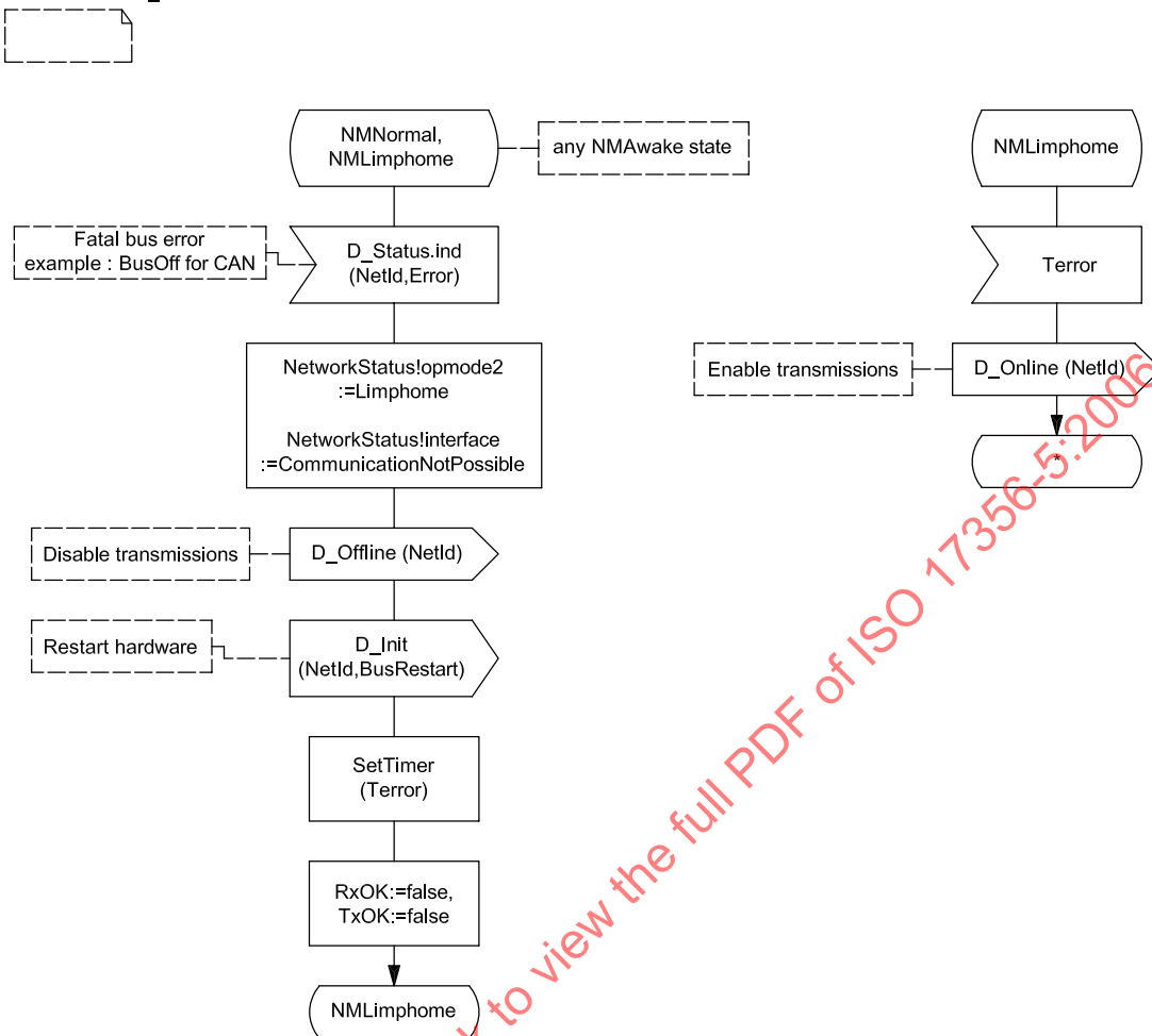
Figure 53 — Handling of a fatal bus error
