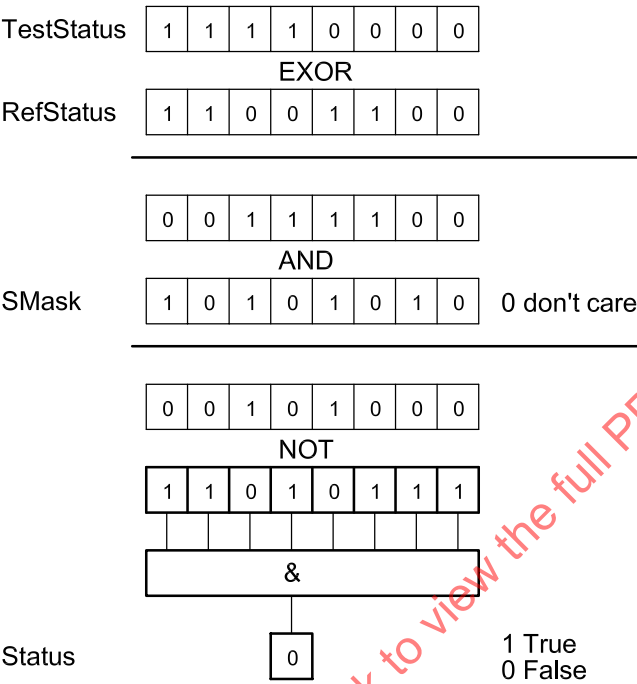
Figure 69 — Example of CmpConfig
