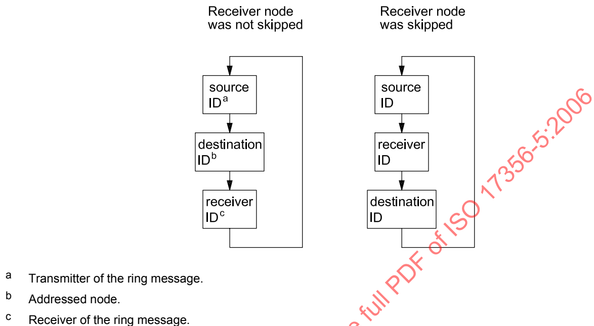
Figure 17 — Temporary logical ring for the test, whether the receiver node has been skipped or not
