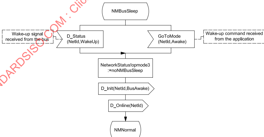
Figure 61 — Handle the transition from NMBusSleep into NMNormal
