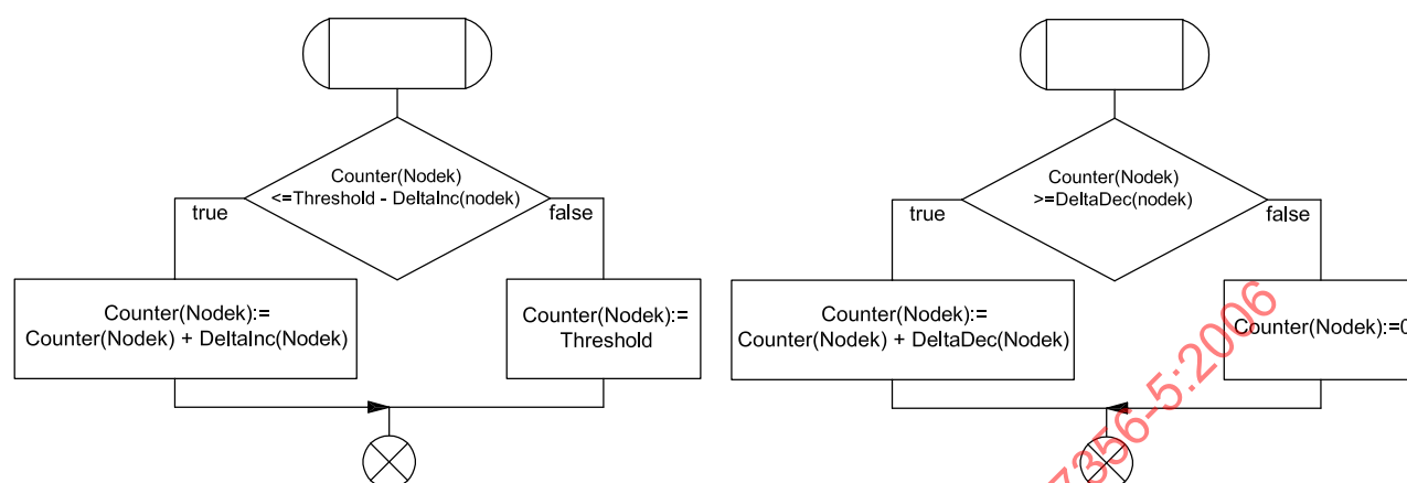
Figure 64 — Decrement and increment procedures for the extended configuration
