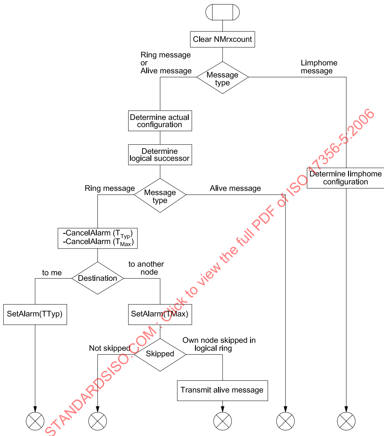
Figure 13 — Actions during NMNormal in case an NM message is received “at a time”
