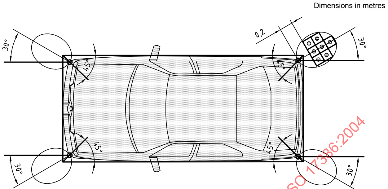
Figure 5 — “Brick definition” of vehicle corners and minimum corner detection ranges
