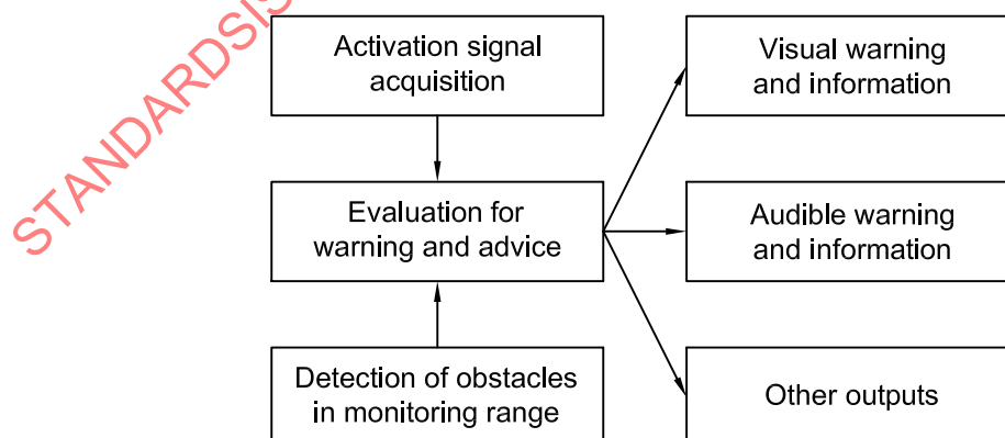
Figure 2 — Block diagram of the potential sub-functions of a manoeuvring aid for low-speed operation.
