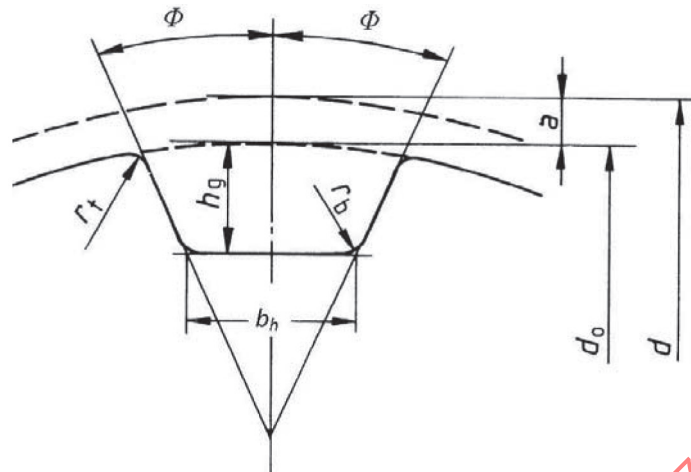
Figure 6 — Profile system AT — Pulley groove profile
