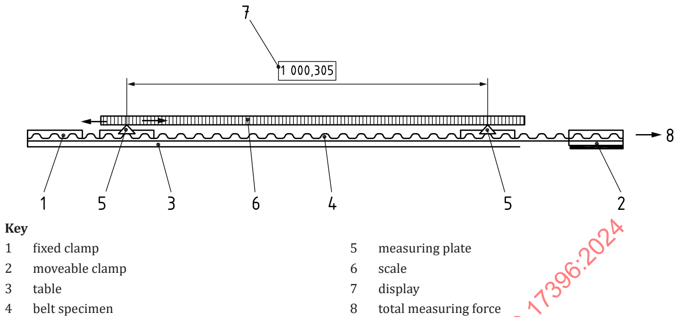
Figure 3 — Fixture for measuring pitch length of very long endless belts and open belts
