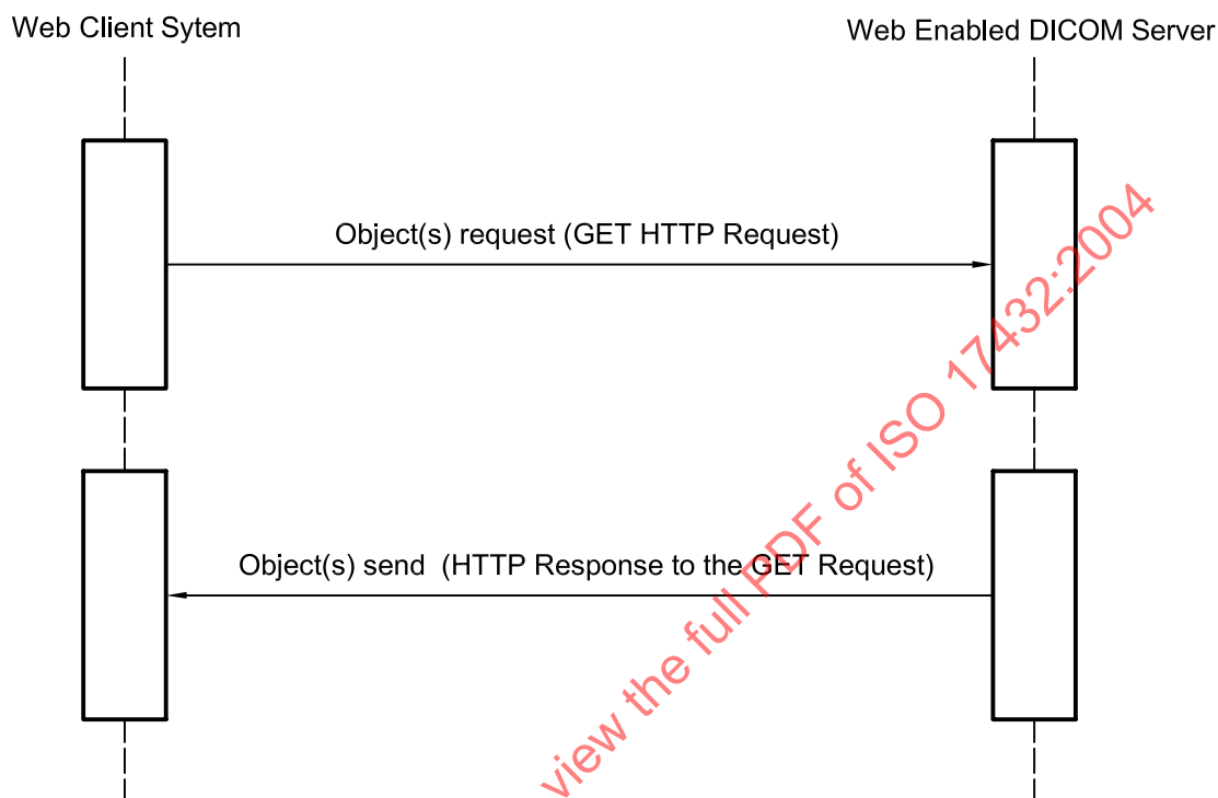
Figure 1 — Interaction diagram
