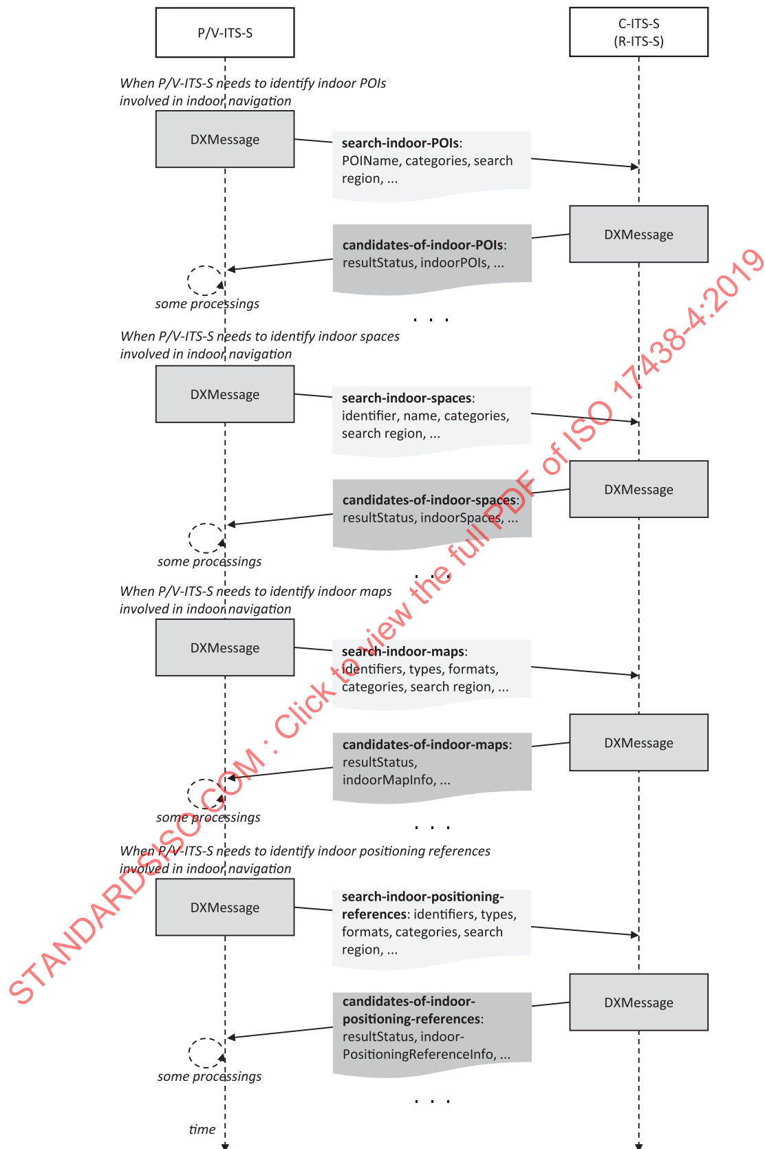
Figure 2 — Message flow
