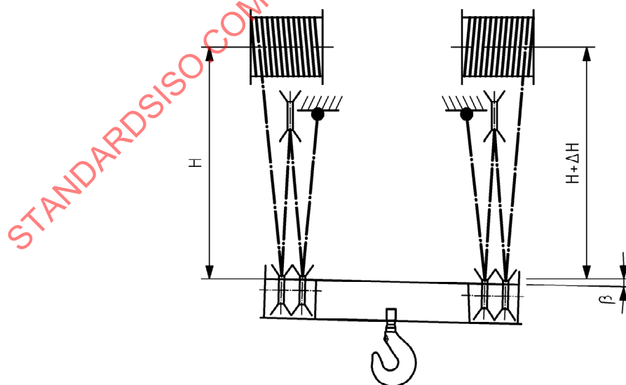
Figure 3 — Tilting of a hook in case of different hoist travel distances
