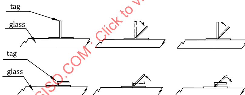
Figure 2 — One time bending (forward and backward)
