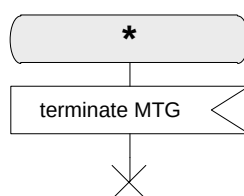
Figure 178 — Termination of the MTG process [MTG]
