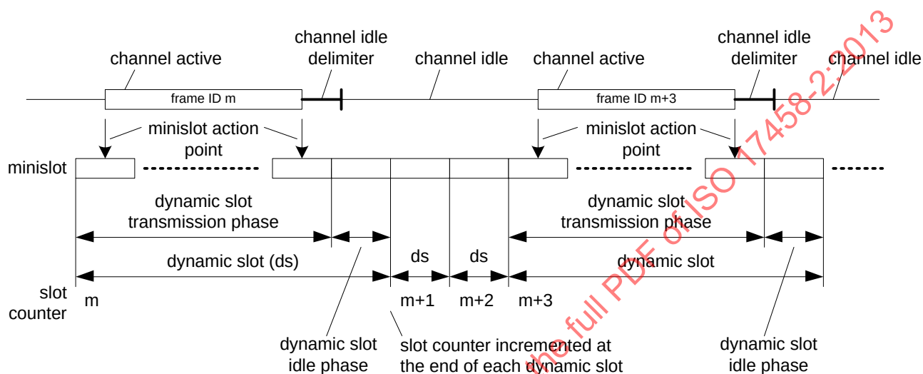
Figure 89 — Structure of dynamic slots
