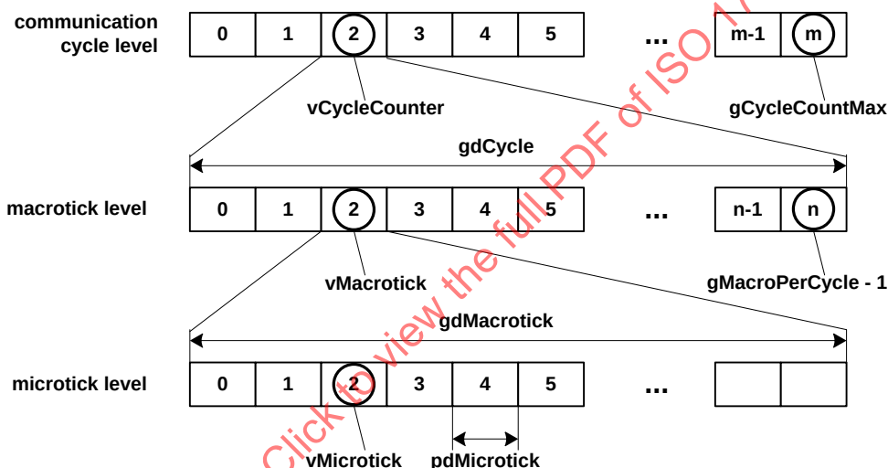
Figure 153 — Timing hierarchy
