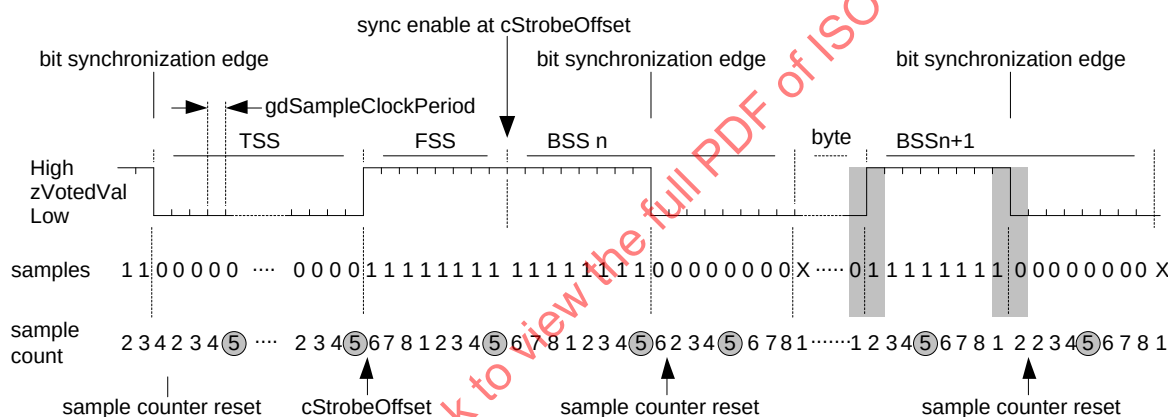
Figure 45 — Bit synchronisation
