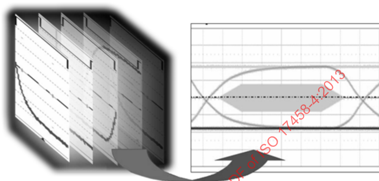
Figure A.20 — Generation of FlexRay eye-diagrams
