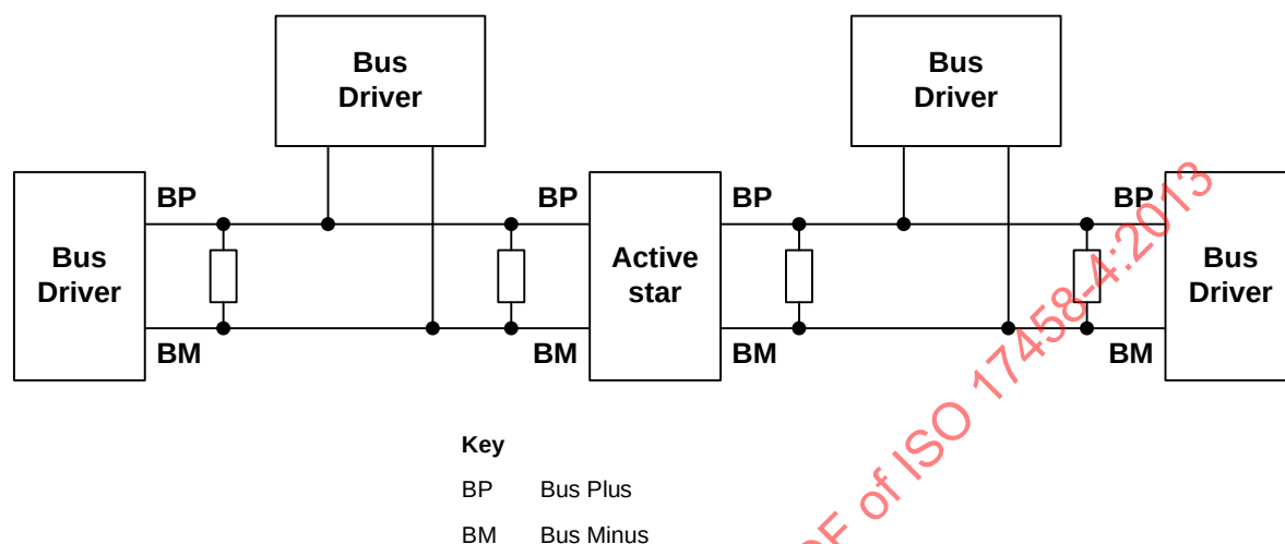
Figure 10 — Principle of an active star network
