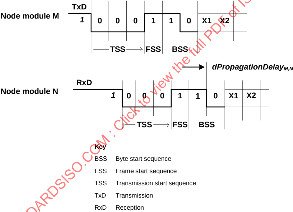
Figure 2 — Propagation delay
