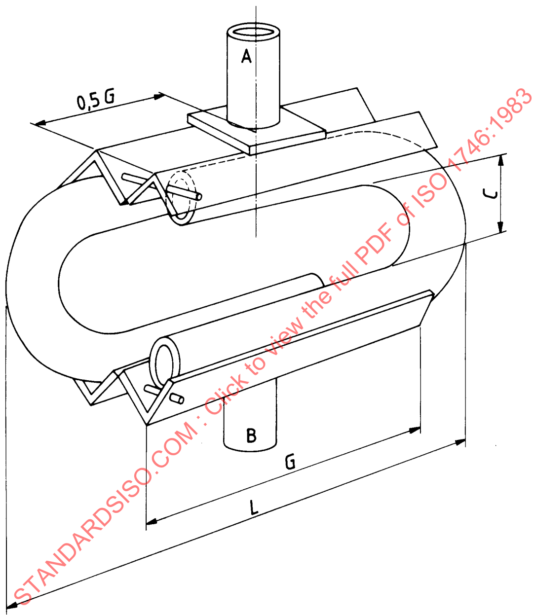
Figure 4 — Schematic arrangement for method B
