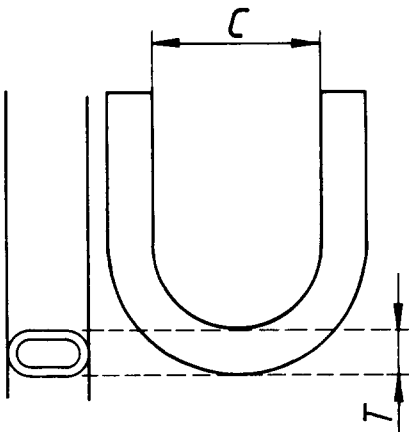
Figure 3 — Measurement of coefficient of deformation
