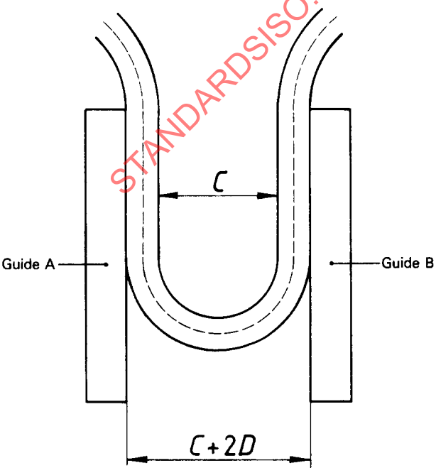
Figure 2 — Schematic arrangement for method A
