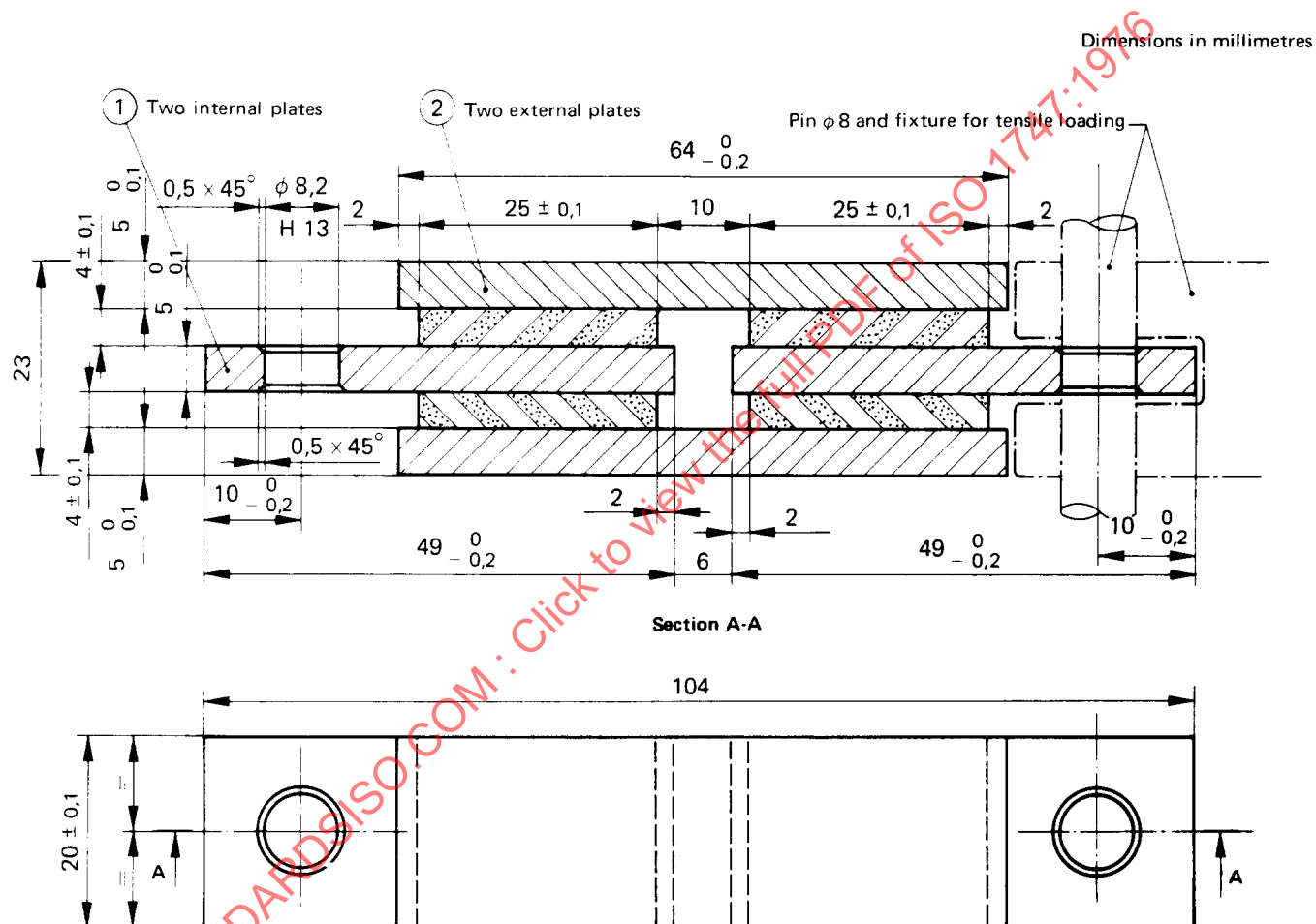
FIGURE 1 – Test piece
