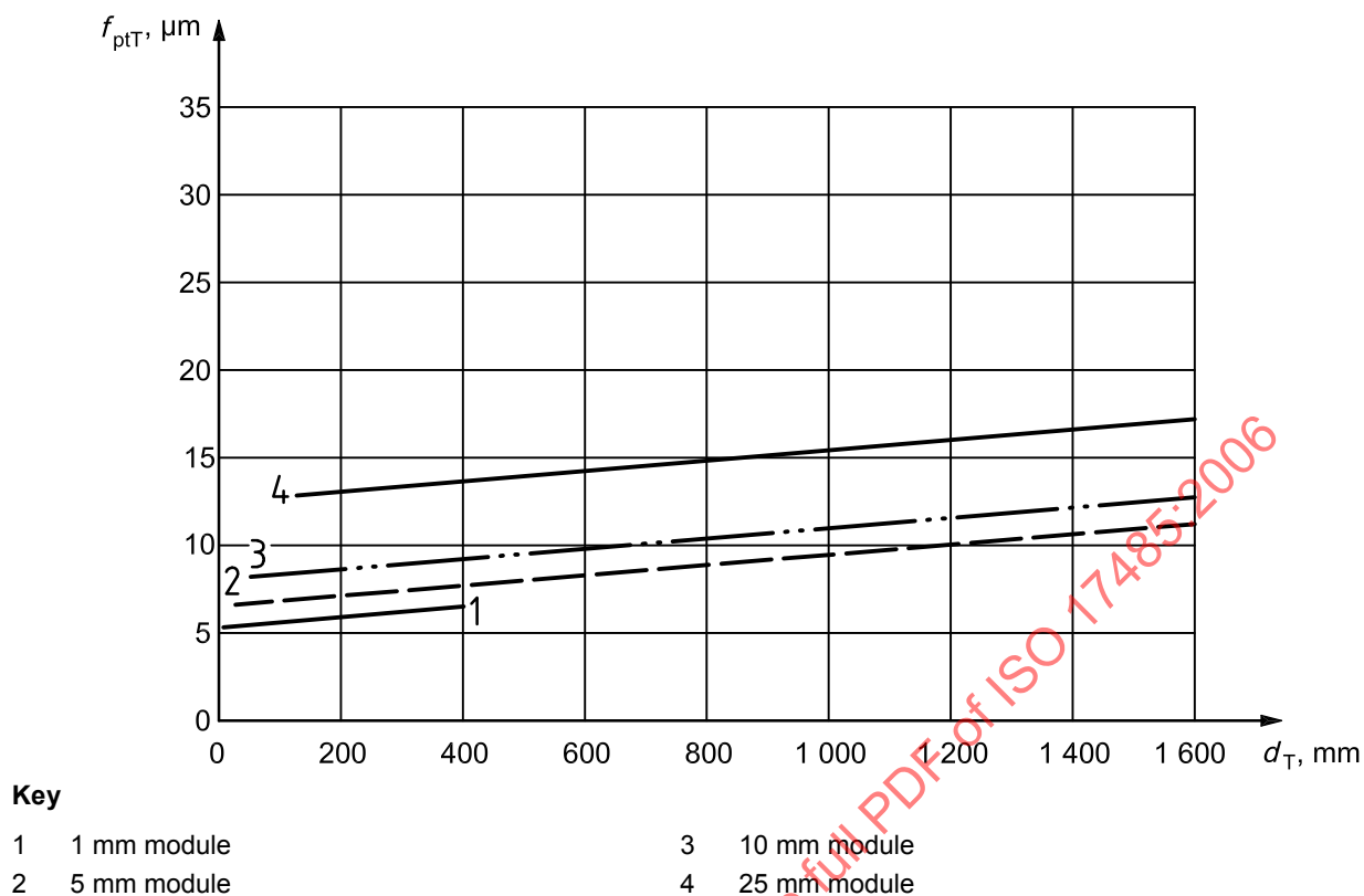
Figure A.1 — Single pitch tolerance, f_{ptT} , grade 4
