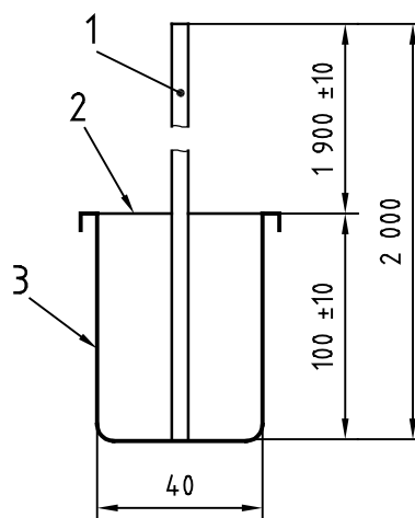
Figure 7 — Arrangement of collecting graduated beaker or cylinder
