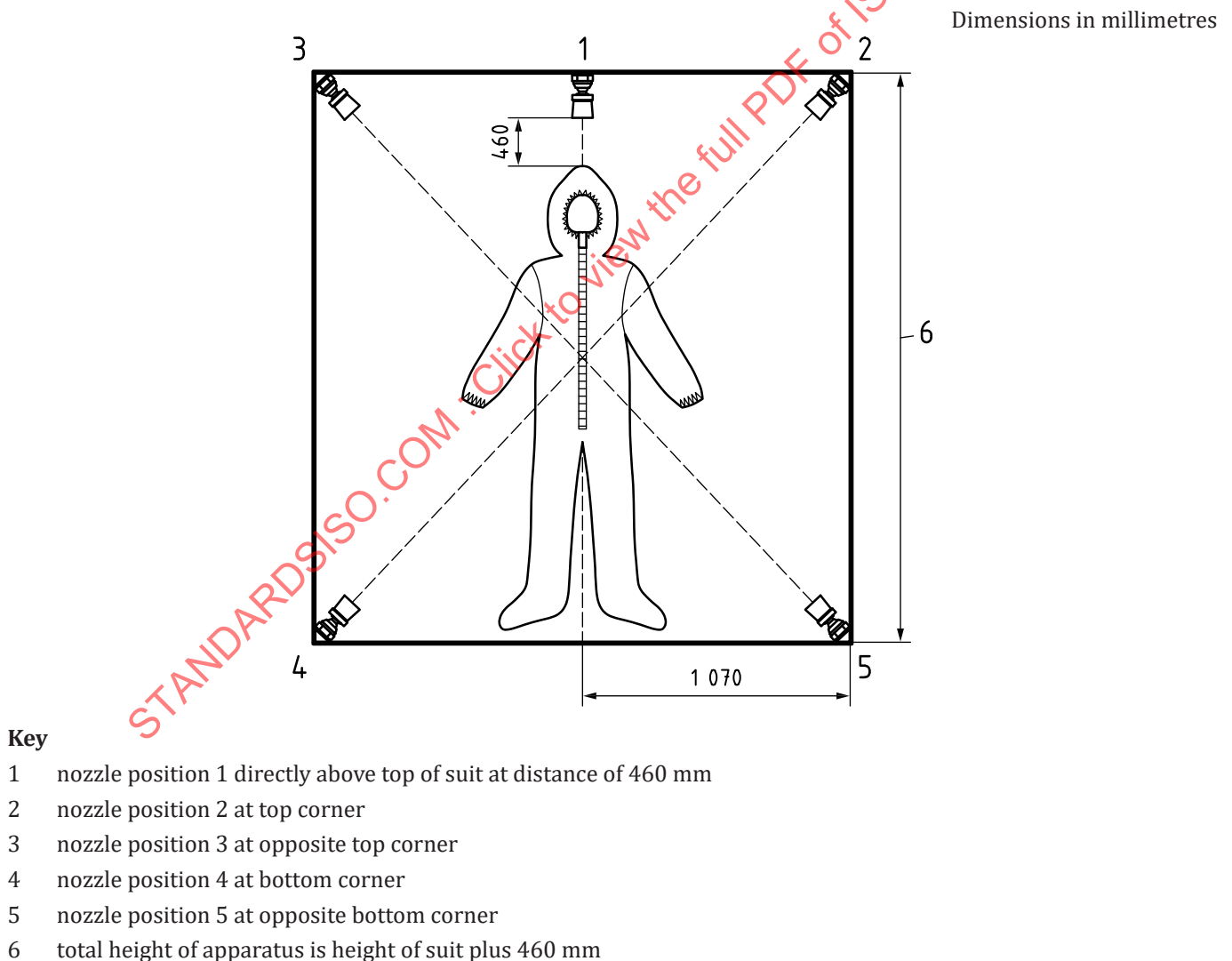
Figure 2 — Positions of shower nozzles (front view)
