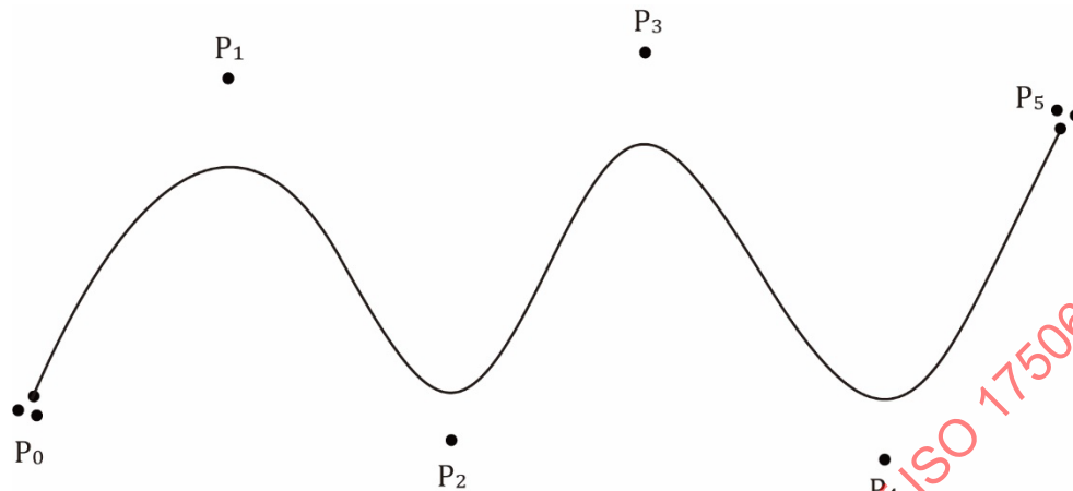
Figure 4 — Example of B-splines
