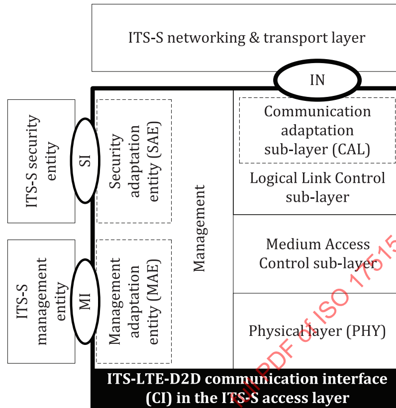
Figure 10 — LTE-D2D CI architecture
