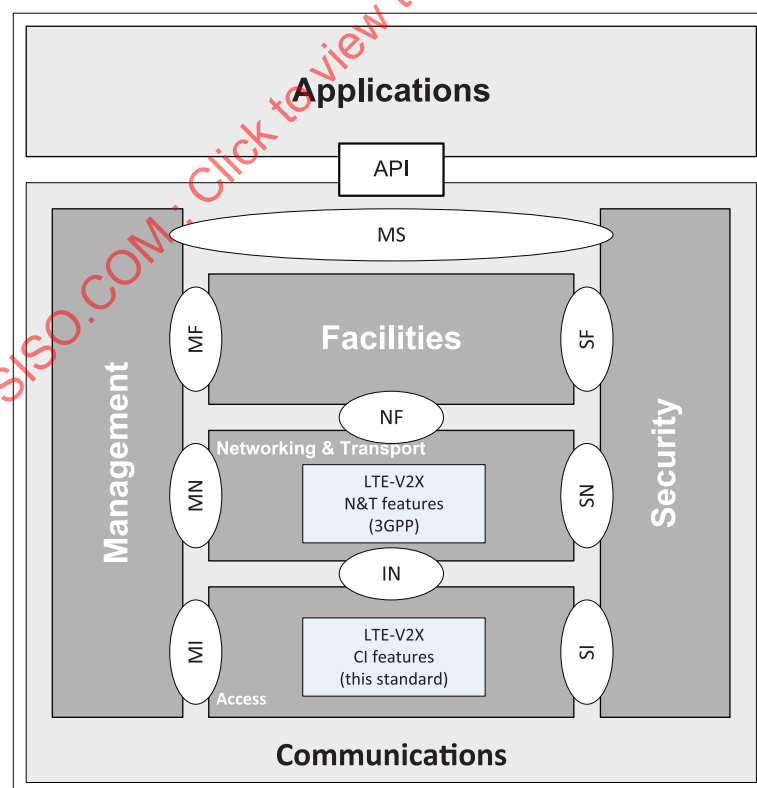
Figure 3 — LTE-V2X functionality in an ITS station
