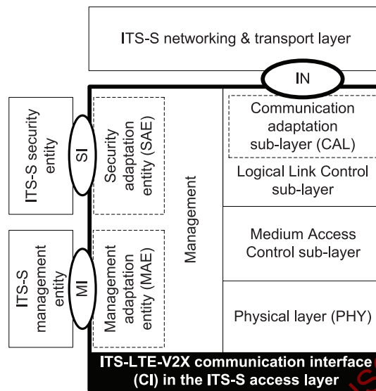
Figure 2 — LTE-V2X CI architecture
